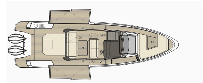
03 Main deck with aft cabin
